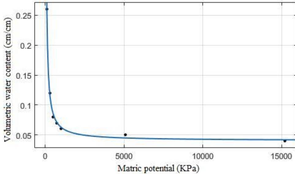
Figure 1. Water retention curve of the soil for the field site
