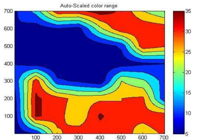
Figure 10. Electrical bio-impedance tomography picture for skin exposed to US, 3 W /cm 2 , for 4 min: 2D linear data interpolation with the size of (700x700) data elements.
