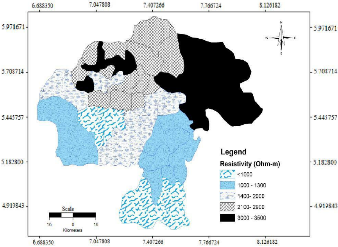
Figure 6. Thematic map of the Imo River basin showing layer of average resistivity
