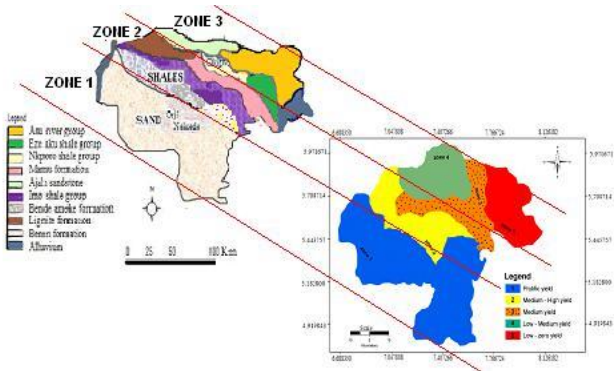
Figure 10. Correlation of Regional geology with the groundwater prospect model.
