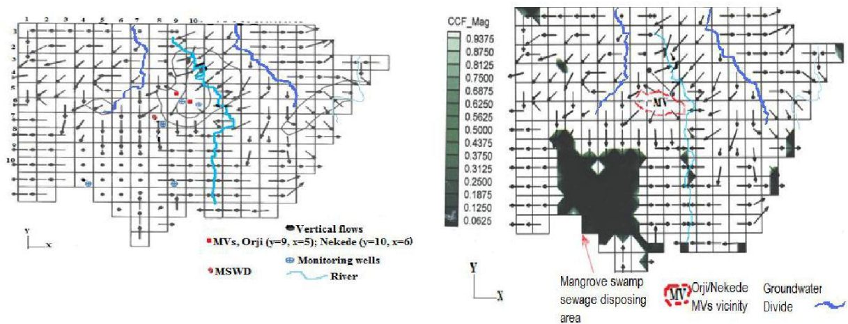
Figure 2. Groundwater flow model by MODFLOW model code, show direction of groundwater flow south of Imo River basin
