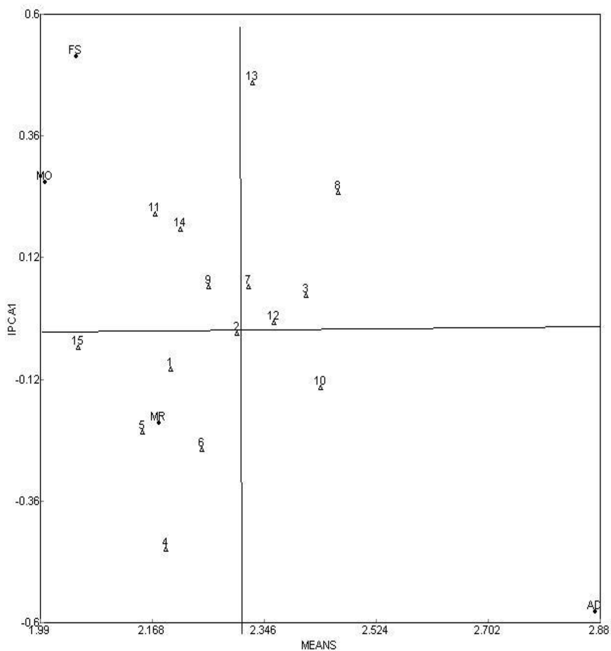
Figure 1. AMMI 1 biplot for grain yield of maize genotypes showing means of genotypes (numbers) and environments (upper case letters) plotted against their IPCA1 scores.
