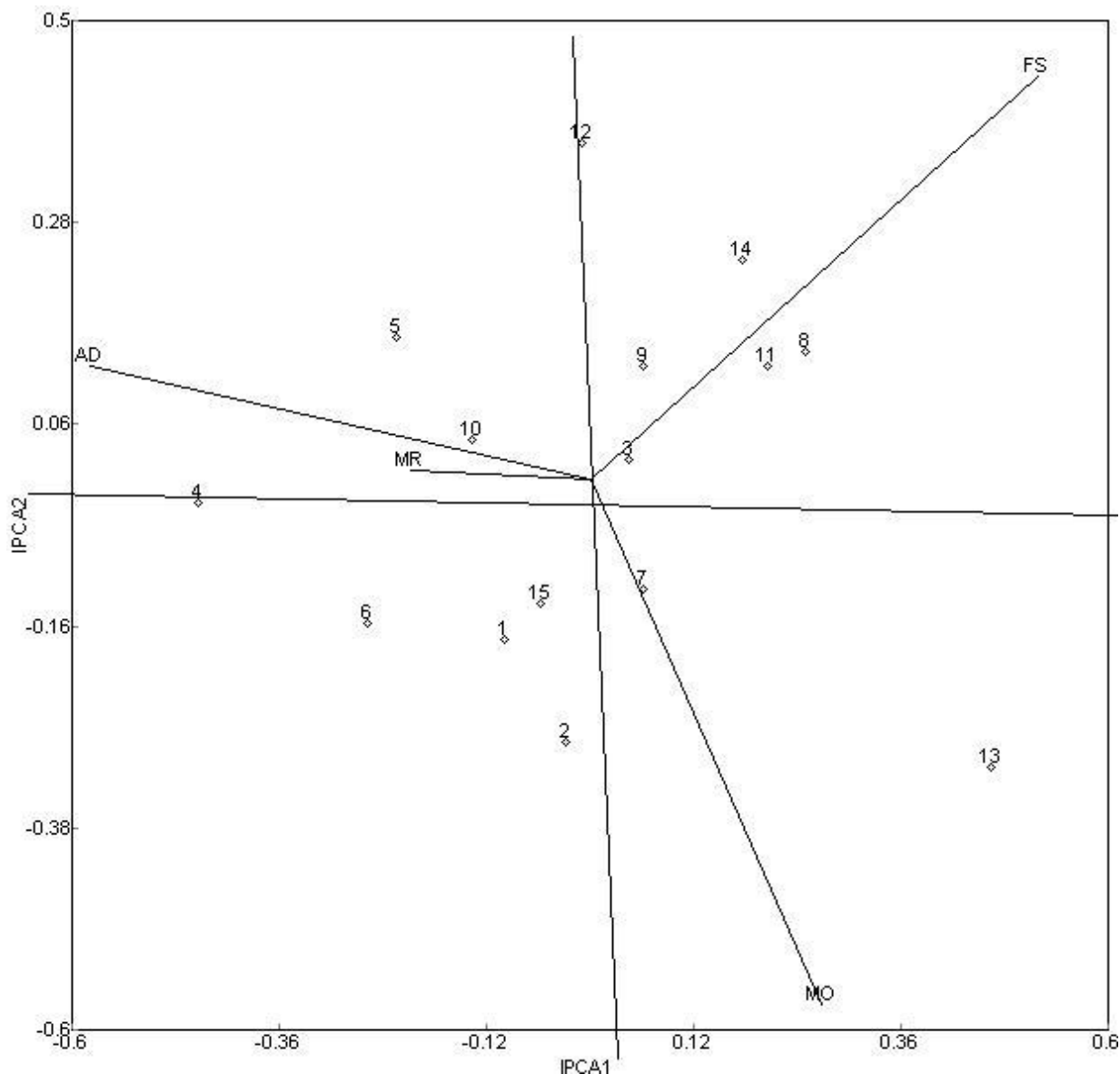
Figure 2. AMMI 2 biplot for grain yield of maize genotypes showing the plotting of IPCA1 and IPCA2 of genotypes. 1= BHQP-542, 2= BH-543, 3= BHQPY-545, 4= GIBE-1, 5= BH-660, 6= BH-670, 7= BH-540, 8= JIBAT-851, 9= HORRA, 10= WONCHI, 11= ARGENE, 12= Phb-30D79, 13= Phb-3253, 14= Phb-30G19, 15= Phb-30H83.
