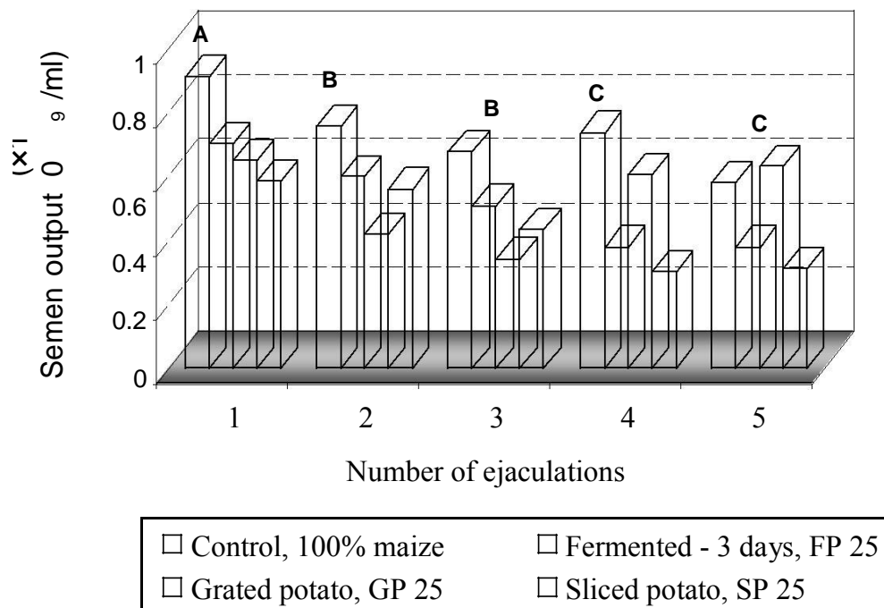
Figure 2. Effect of feed and ejaculation frequency on semen output, frequencies of ejaculation with different superscripts (A, B or C) were significantly different ( P < 0.05 ).
