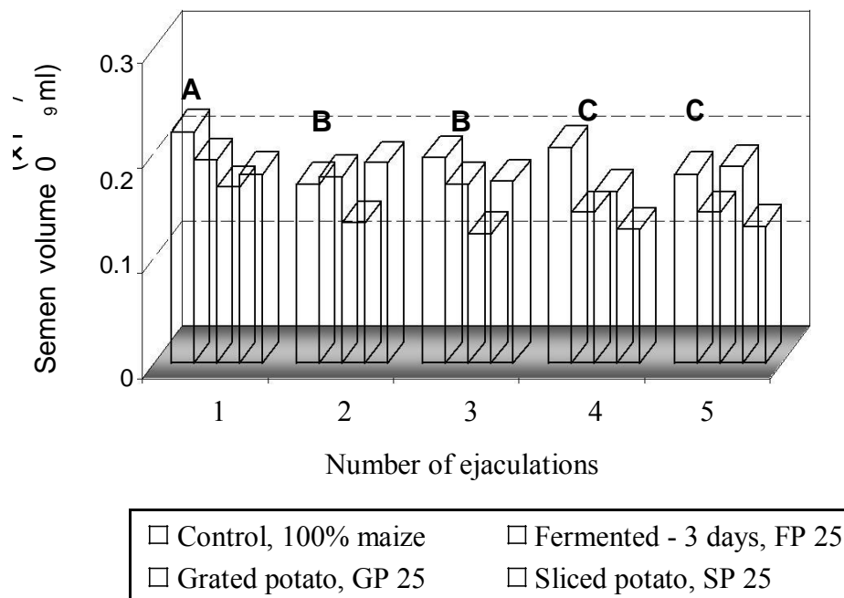
Figure 1. Effect of feed and ejaculation frequency on semen volume. Frequencies of ejaculation with different superscripts (A, B, C or D) were significantly different ( P < 0.05 ).
