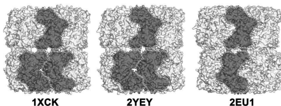
Figure 2. Comparison between wild-type GroEL, GroEL E434K and GroEL E461K mutants. In both wild-type GroEL (PDB 1XCK) and GroEL E434K (PDB 2YEY), each protomer contacts two protomers at the opposing ring (1:2 contact). In contrast, in the GroEL E461K mutant (PDB 2EU1), the upper ring is rotated 22° about the 7-fold axis, and consequently each protomer contacts only one protomer at the opposite ring (1:1 contact).
