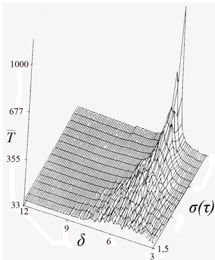
Figure 2. simulation results of the model in which the average elimination time, \bar{T} , is plotted as a function of variance in the generation time, \sigma(\tau) , for regimens that differ in
