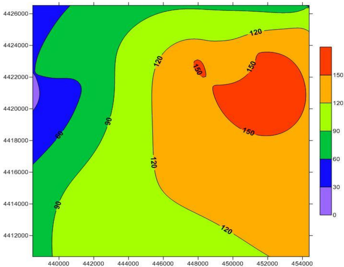
Figure 5. Spatial distribution of nitrate concentration for 2010 (mg/L).
