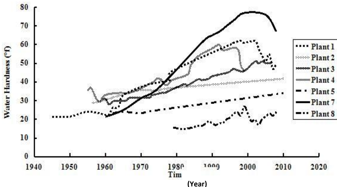
Figure 7. Changes of hardness with time.
