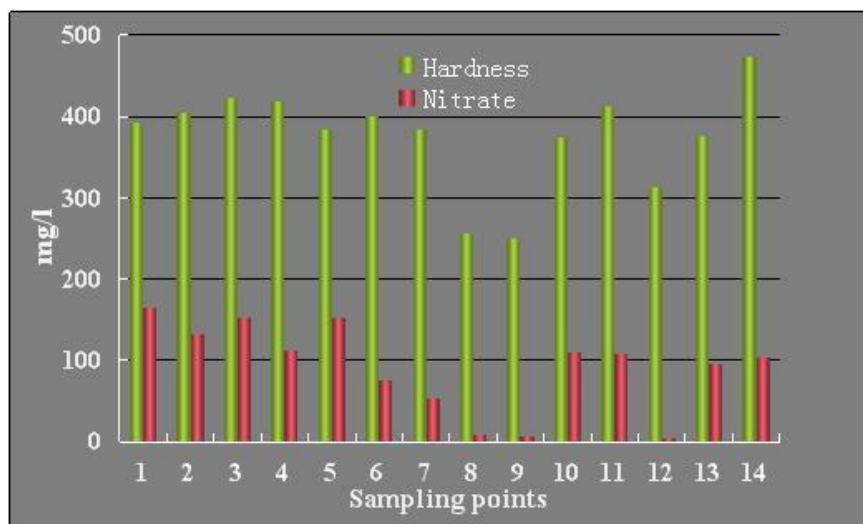
Figure 6. Relationship between hardness and nitrate concentrations.
